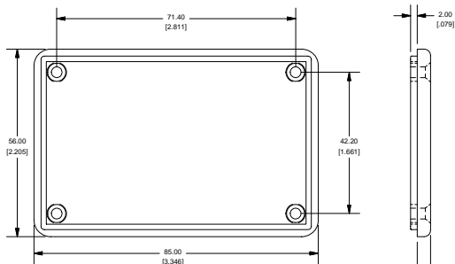
SIDE VIEW OF LID
